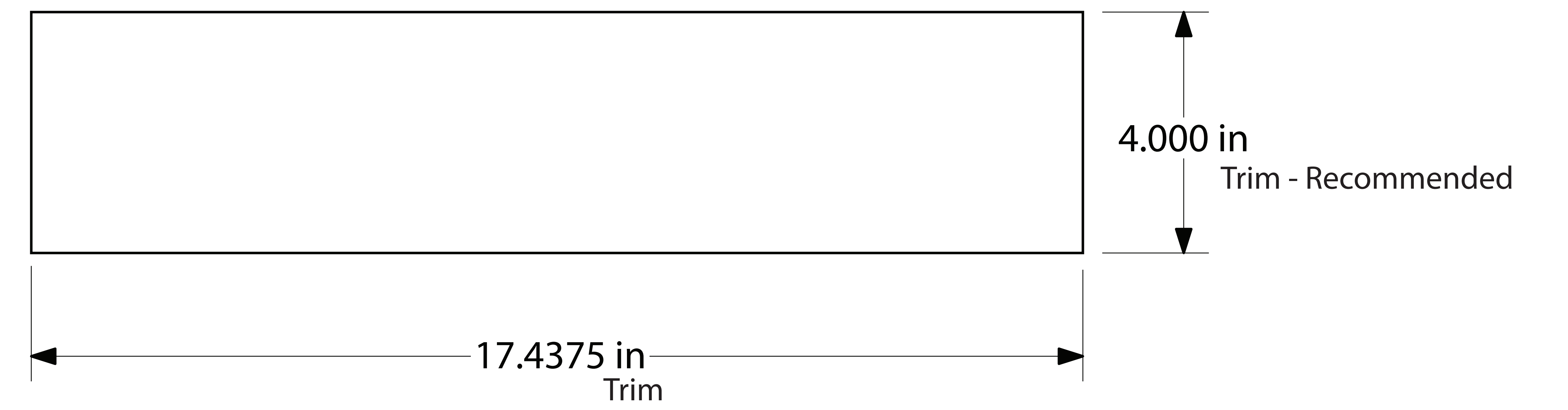
DOOR DECAL OC6 Artwork - Recommended Substrate Thickness: 0.004"
